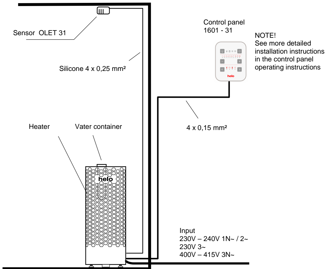
Principle image
