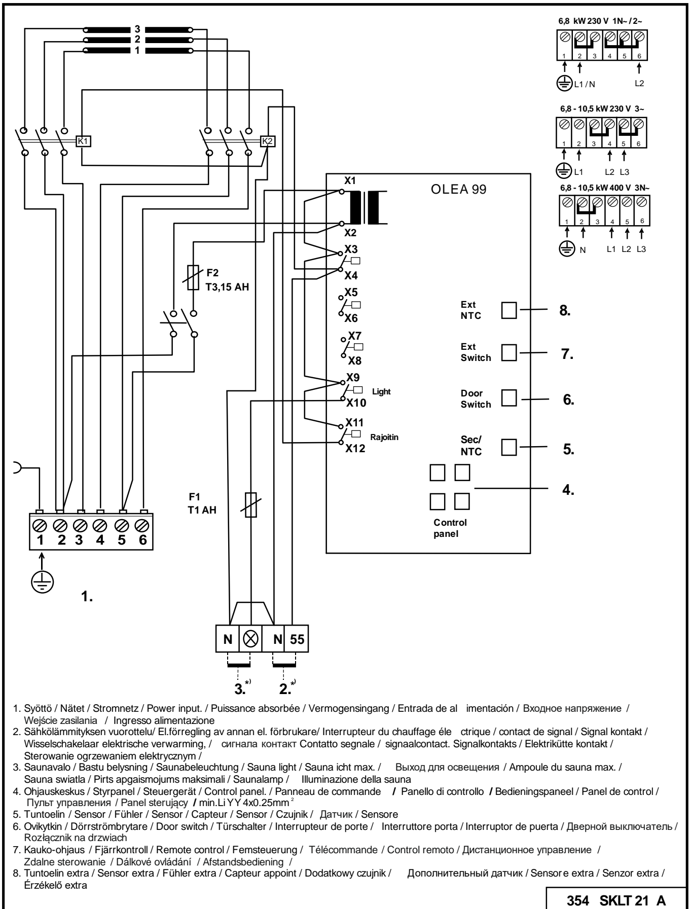
Figure 6 Wiring diagram for the sauna heater
