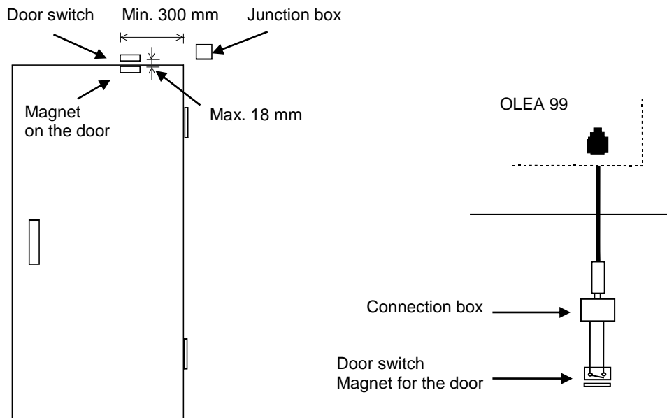
Figure 4 Installing the door switch
